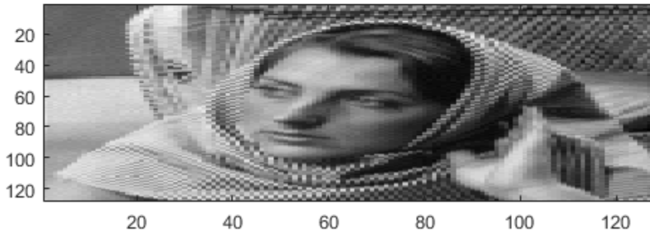
Lowpass Approximation
